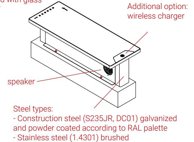
ISOMETRIC VIEW (BACK VIEW)
