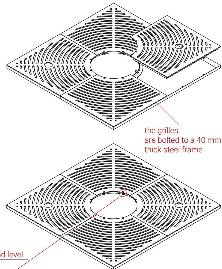
ISOMETRIC VIEW
