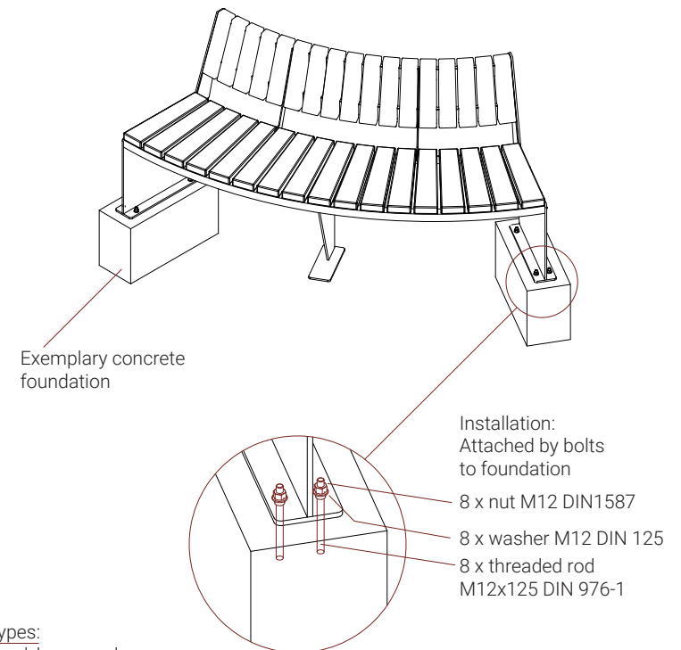
ISOMETRIC VIEW
