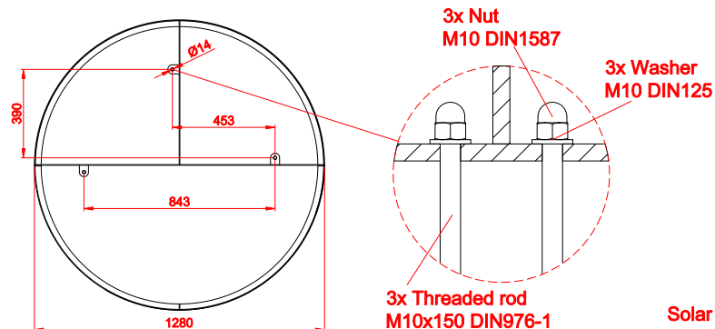
MOUNTING HOLES SPACING
