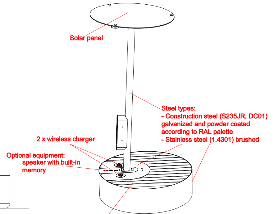
ISOMETRIC VIEW
