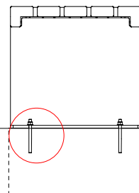
VERTICAL SECTION
