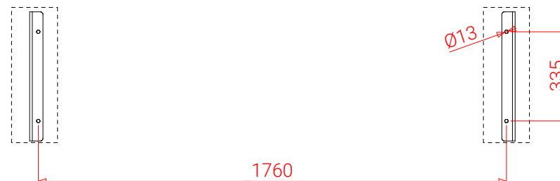
MOUNTING HOLES SPACING
