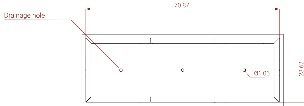
TOP VIEW
