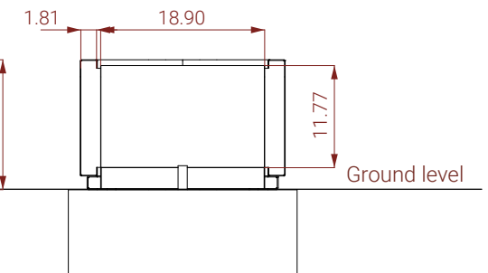
VERTICAL SECTION
