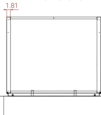
VERTICAL SECTION
