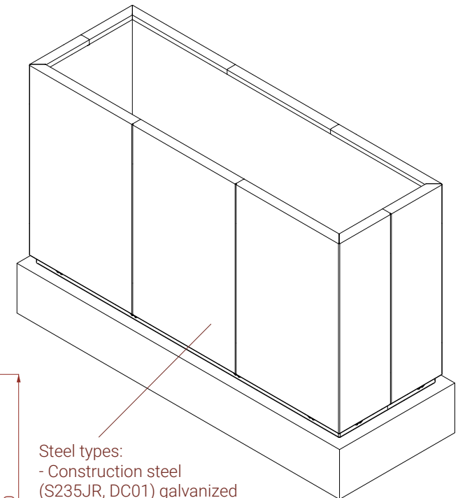
ISOMETRIC VIEW
